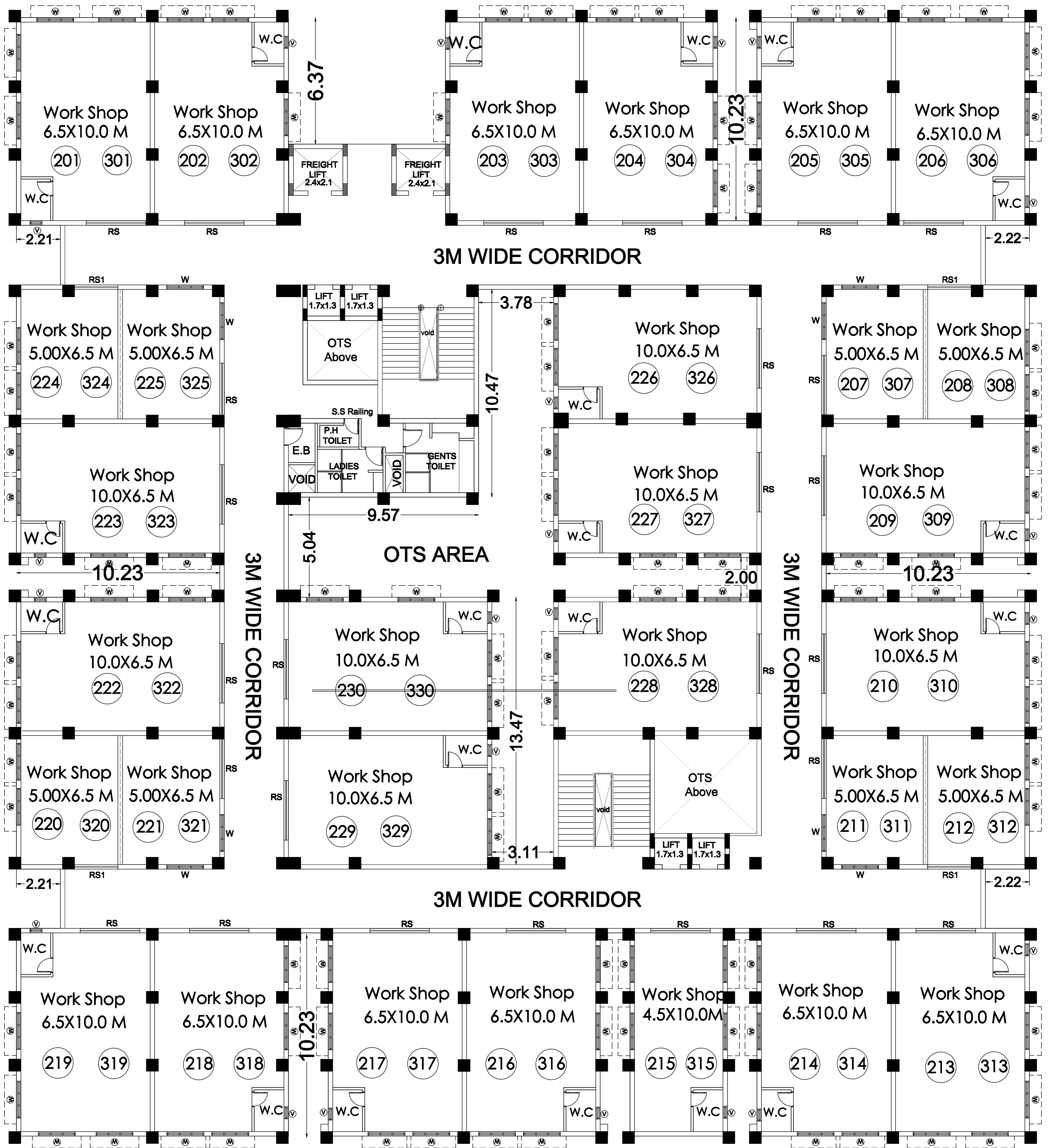
TYPICAL FLOOR PLAN (2 ND FLOOR - 3 RD FLOOR)
